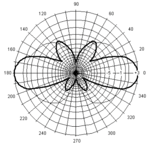
MFB8133 Elevation Pattern
