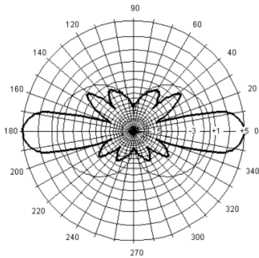
MFB813 Elevation Pattern
