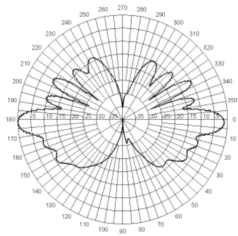
MFB9157 Elevation Pattern
