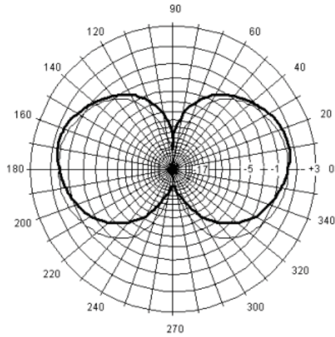
MFB8130 Elevation Pattern
